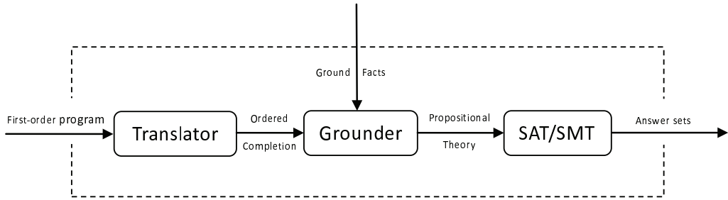
Figure 3: Our new ASP solver
