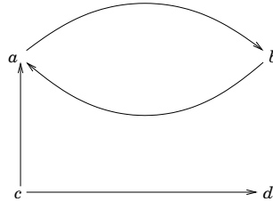
Figure 1: An example graph
