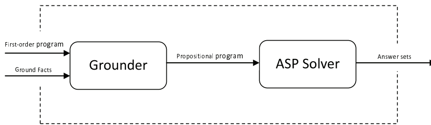
Figure 2: Traditional ASP solvers
