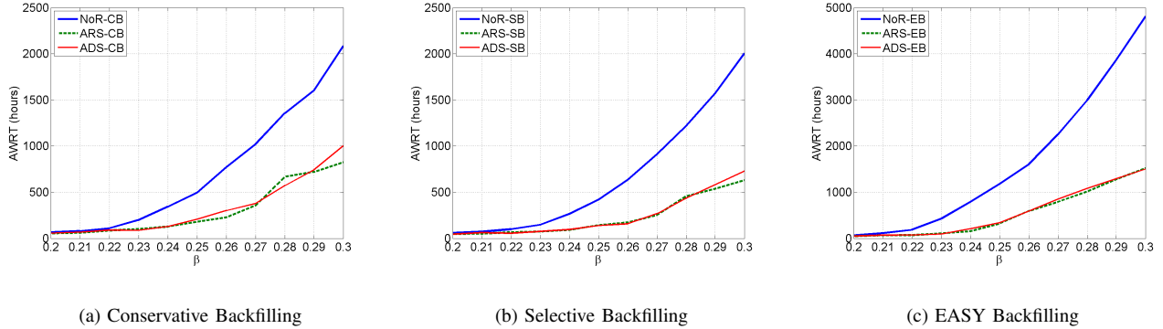
Fig. 3. AWRT versus arrival rate ( \theta = 3.0 ).
