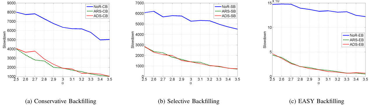
Fig. 6. Slowdown versus request duration ( \beta = 0.25 ).
