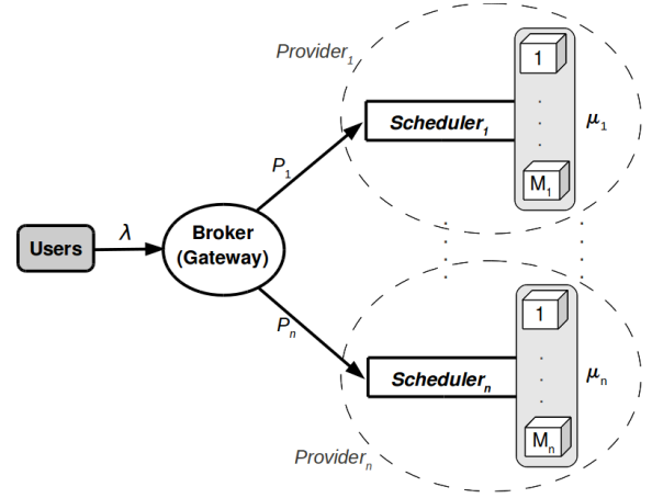
Fig. 2. Model of resource brokering for n providers.
