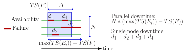
Fig. 2. Parallel and single-node job downtime for a sample space-correlated failure.
