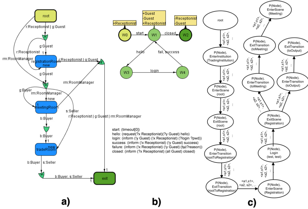
Fig. 2. Institutional Specification and Agent Training.
