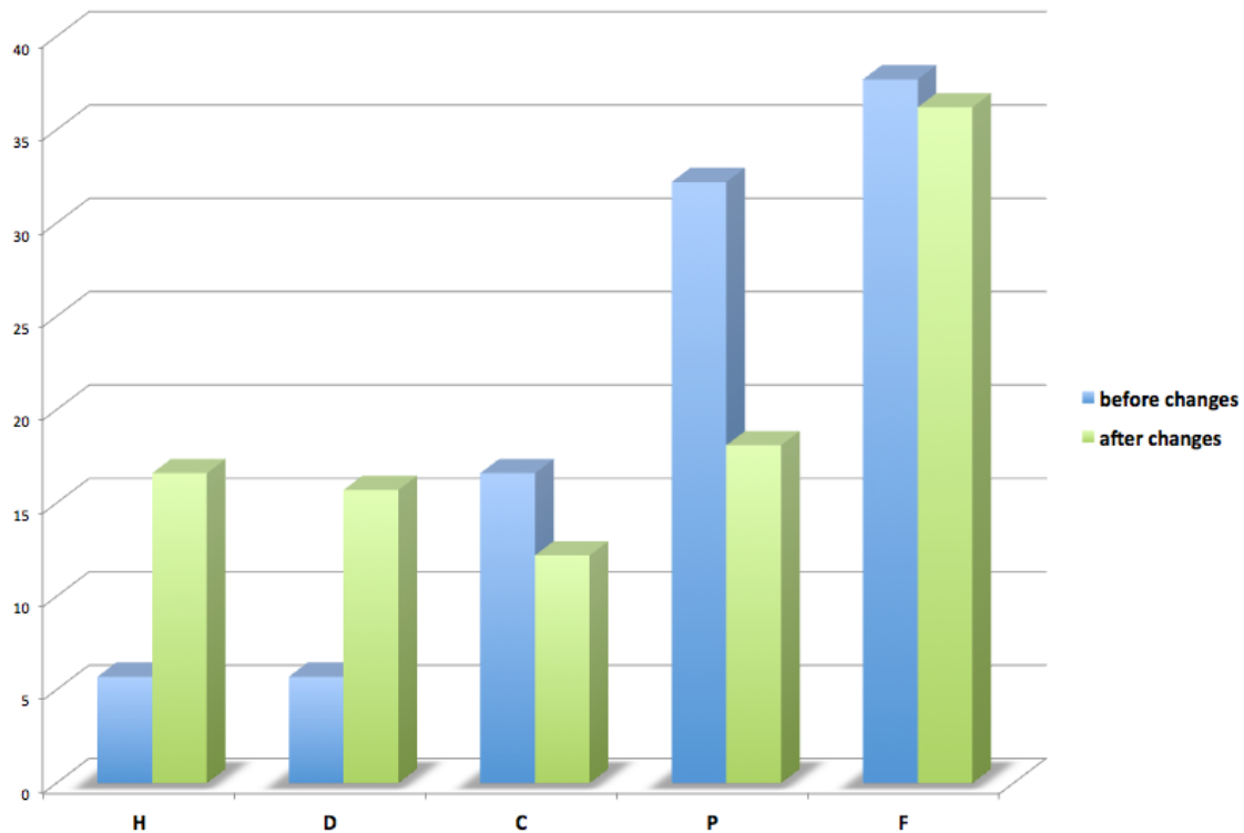
Figure 4: Marks comparison.
