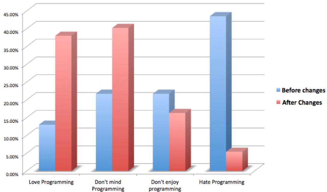
Figure 3: Programming attitude.
